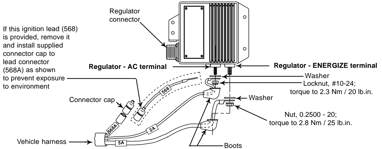
Figure 1a - N3121 Regulator Wiring Connections
