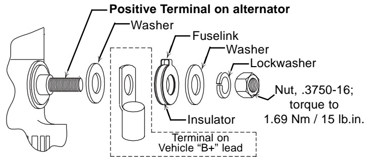
Figure 1a - Positive Terminal Connections
