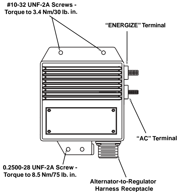
Figure 3 - N3121 Regulator Wiring Connections (also for N1211-5)
