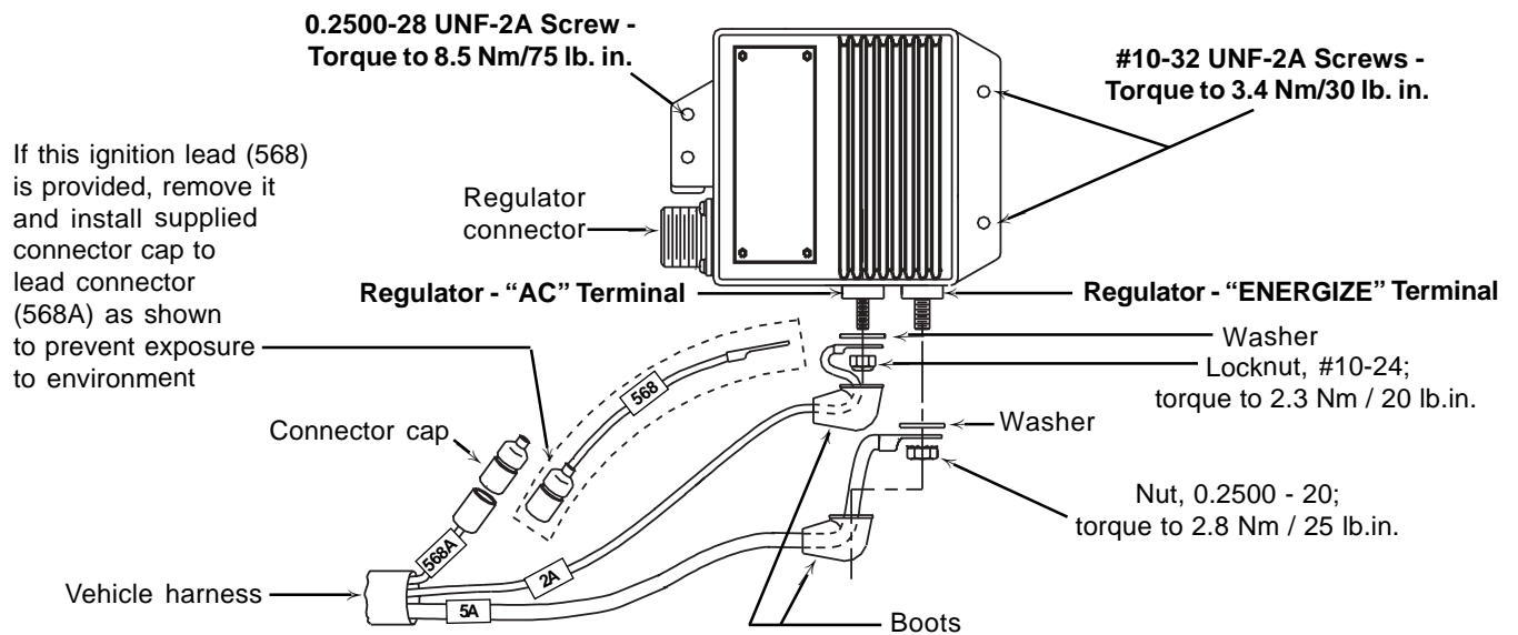
Figure 4 - N3106 Regulator Wiring Connections (also for N1211-2)
