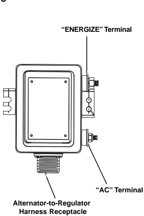
Figure 2 - N3116 Regulator Wiring Connections (also for N1211-4)
