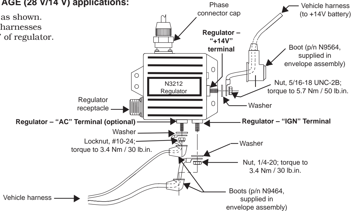
Figure 1 – N3212 Regulator Dual Voltage Wiring Connections
