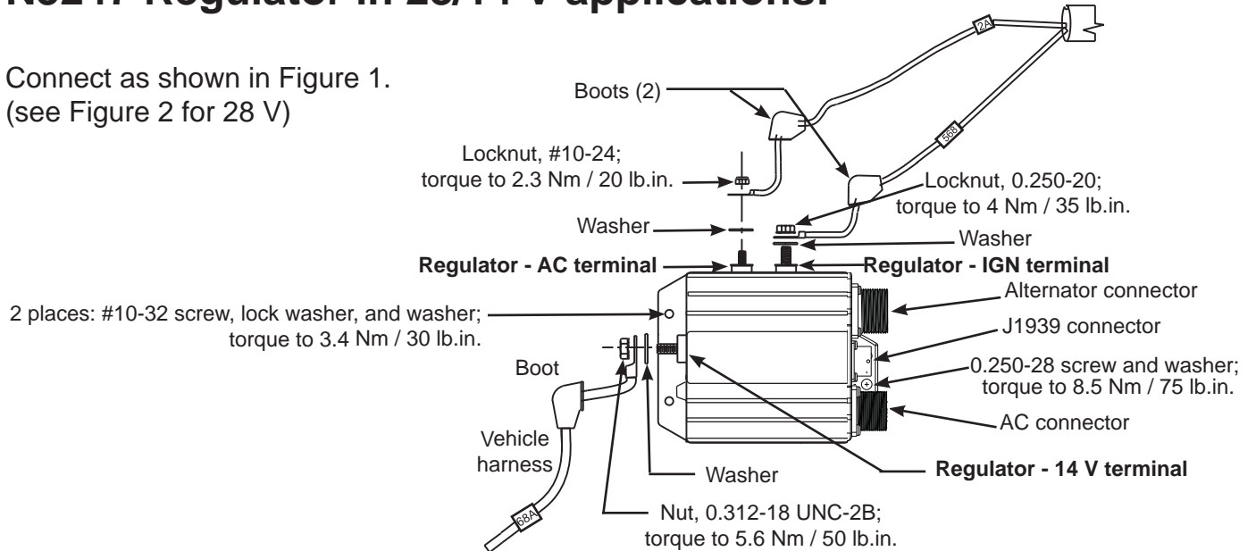
FIGURE 1 – Installing N3247 in 28/14 V Applications
