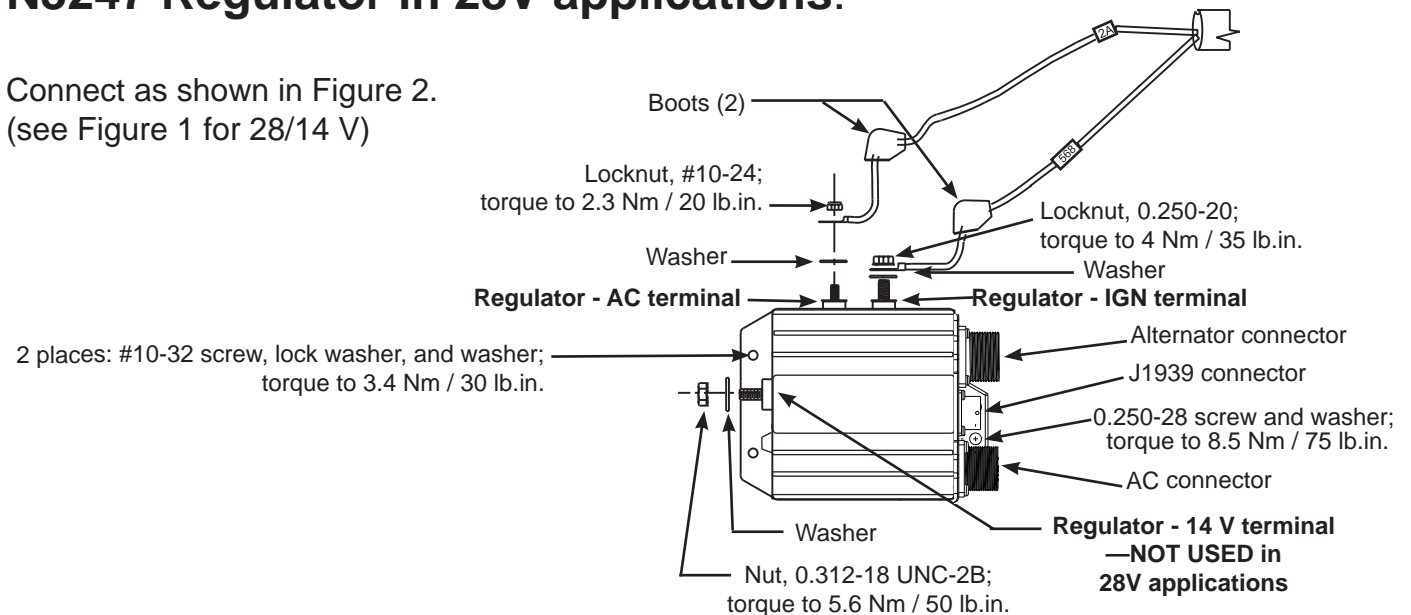
FIGURE 2 – Installing N3247 in 28 V Applications
