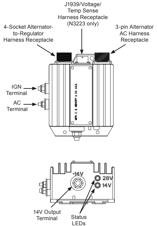
Figure 5: Typical Smart Regulator External Features
