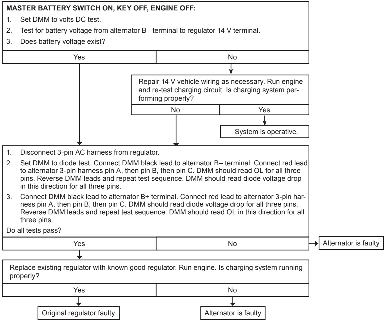
Chart 2: No 14 V Circuit Output
