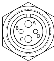
Figure 6: 4-Socket Alternator-to-Regulator Harness Connections
