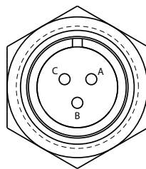
Figure 7: 3-Pin AC Harness Connections
