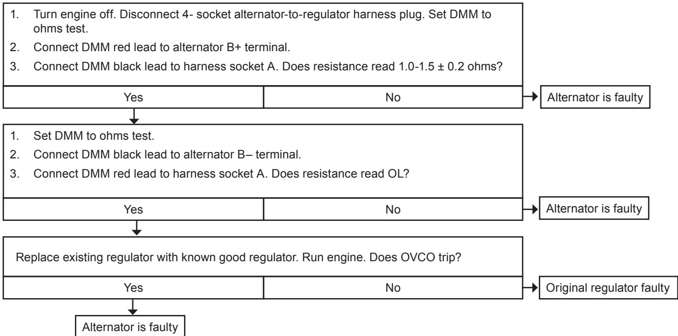
Chart 3: Test OVCO Circuit
