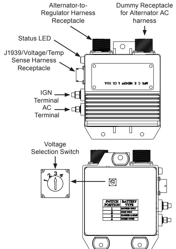
Figure 4: Typical Smart Regulator External Features
