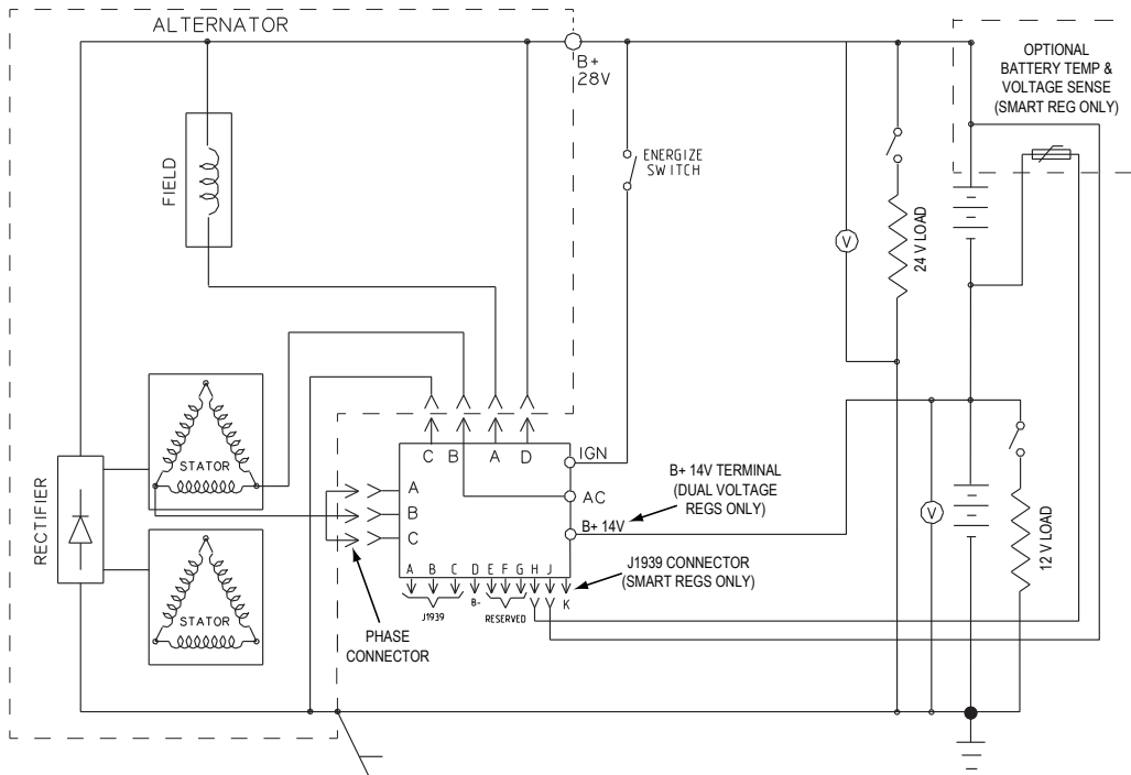
Figure 3: N1602 Alternator Wiring Diagram
