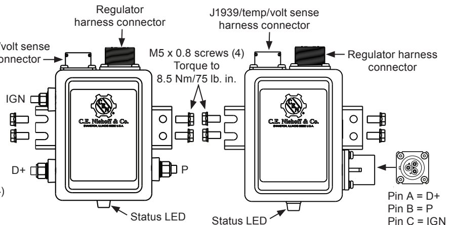
Figure 10: Smart Series Regulator Connections
